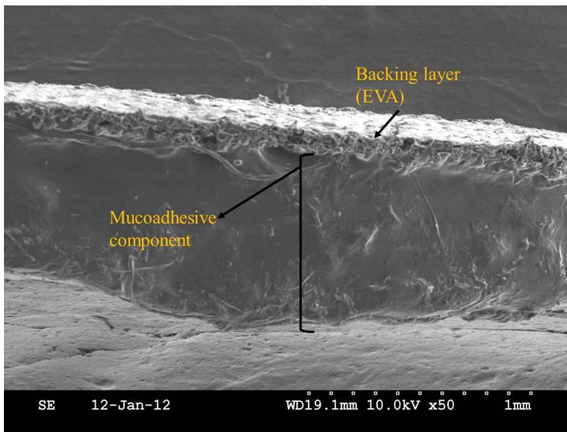
Figure 3.7. Representative scanning electron micrograph showing cross-section of a bilayered mucoadhesive film. The 900- \mu\text{m} -thick mucoadhesive component was backed by a 100- \mu\text{m} -thick PEVA layer.
